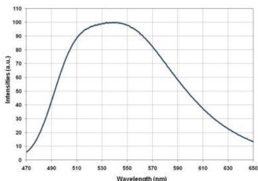
Emission Spectrum
